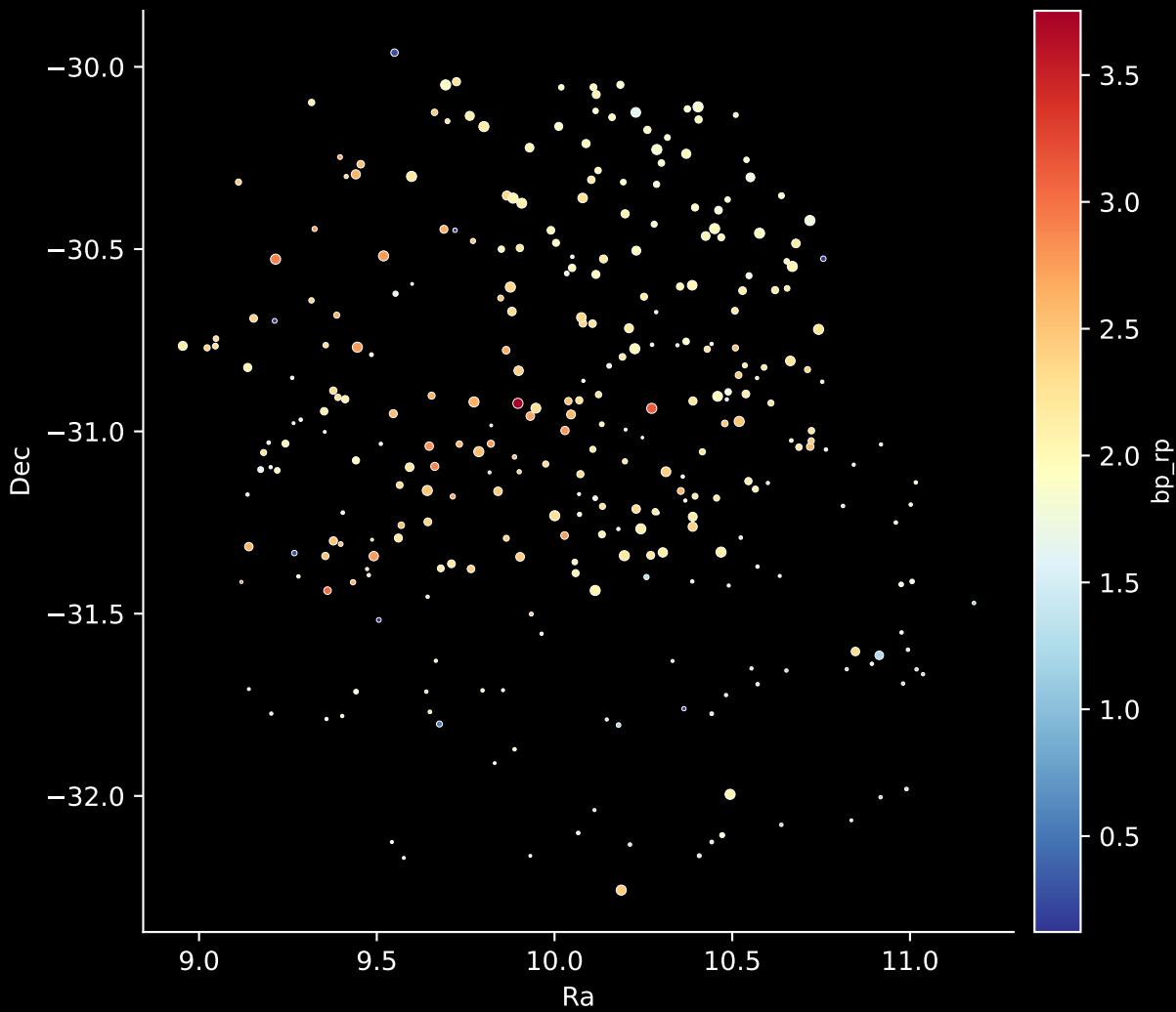
APOGEE DR17 Field: [000-04-O] Stars: 308
