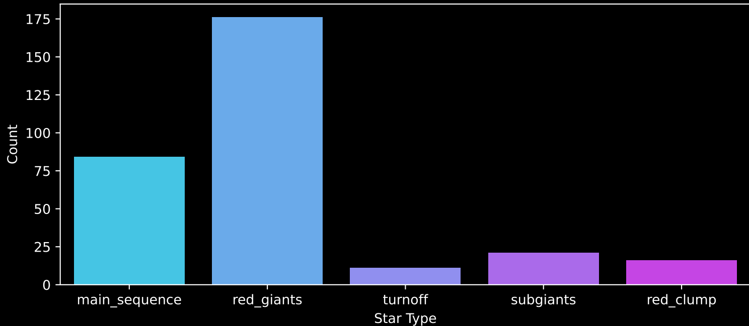
APOGEE DR17 Field: [000-04-O] Count plot of Star Type
