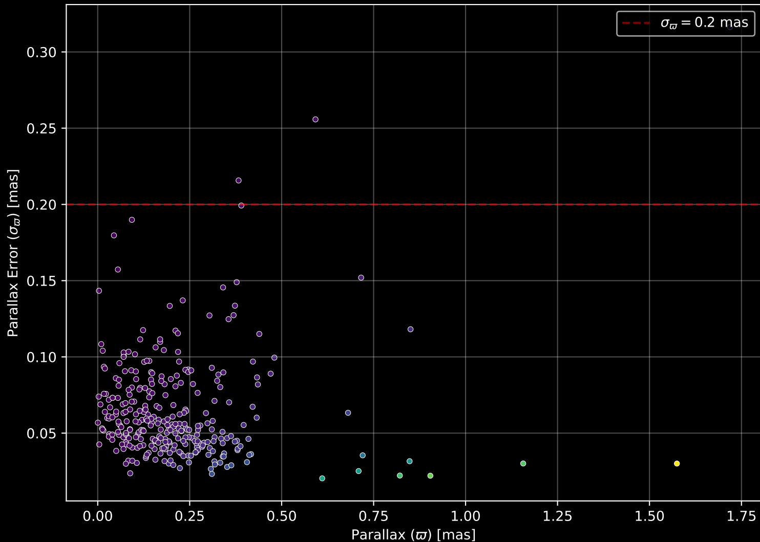
APOGEE DR17 Field: [000-04-O] Parallax Quality (n= 308)
