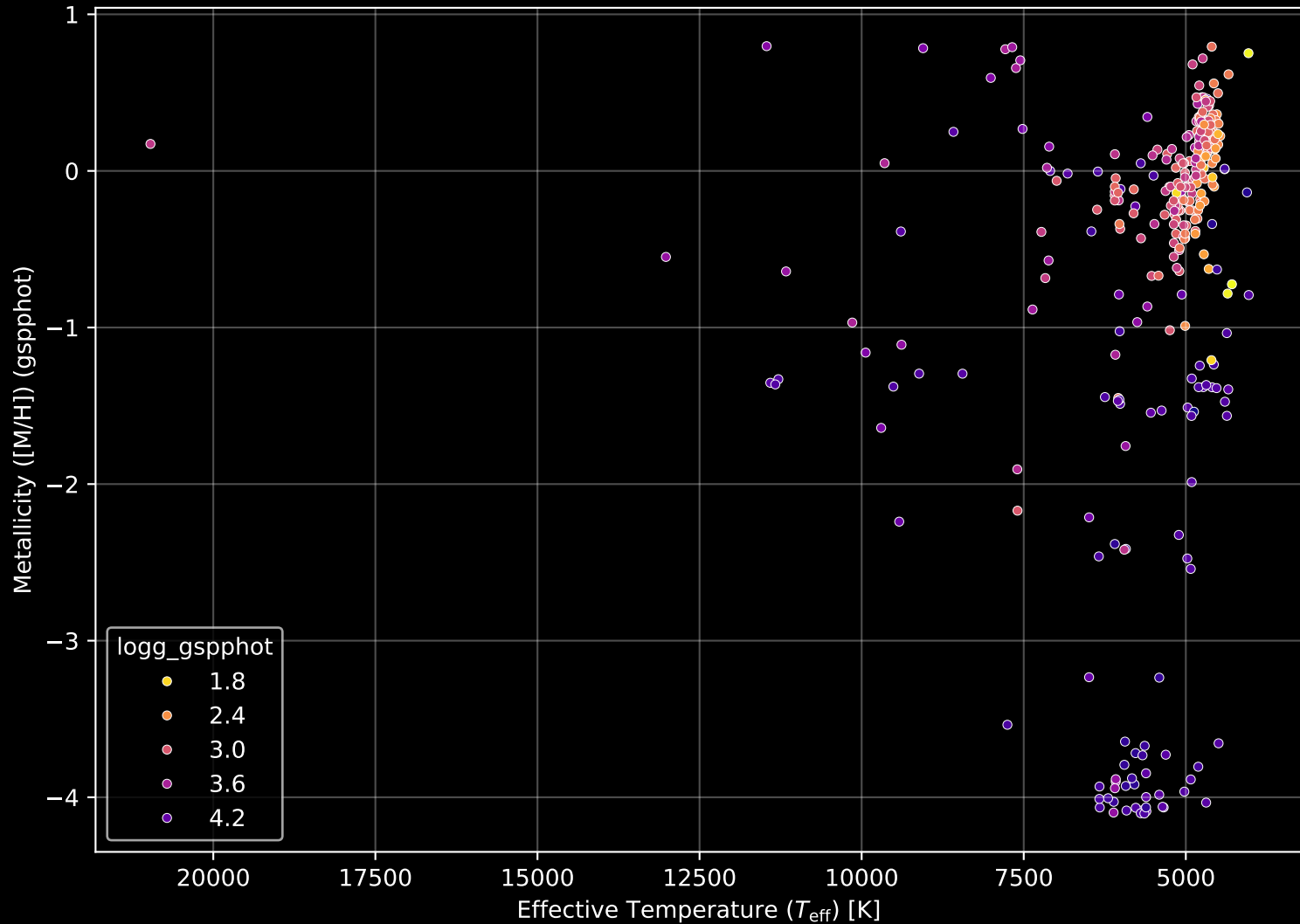
APOGEE DR17 Field: [000-04-O] Stellar Population Parameters (n= 308)
