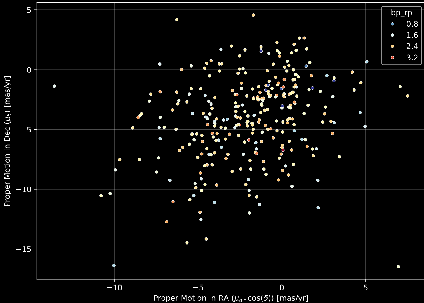
APOGEE DR17 Field: [000-04-O] Proper Motion Diagram (n= 308)
