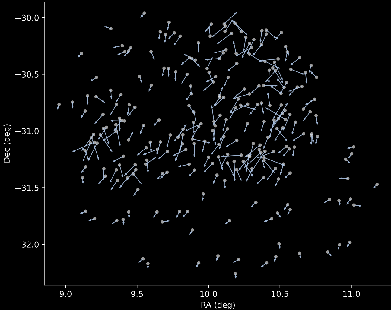
APOGEE DR17 Cluster 1 Proper Motion Vectors (n=251)
