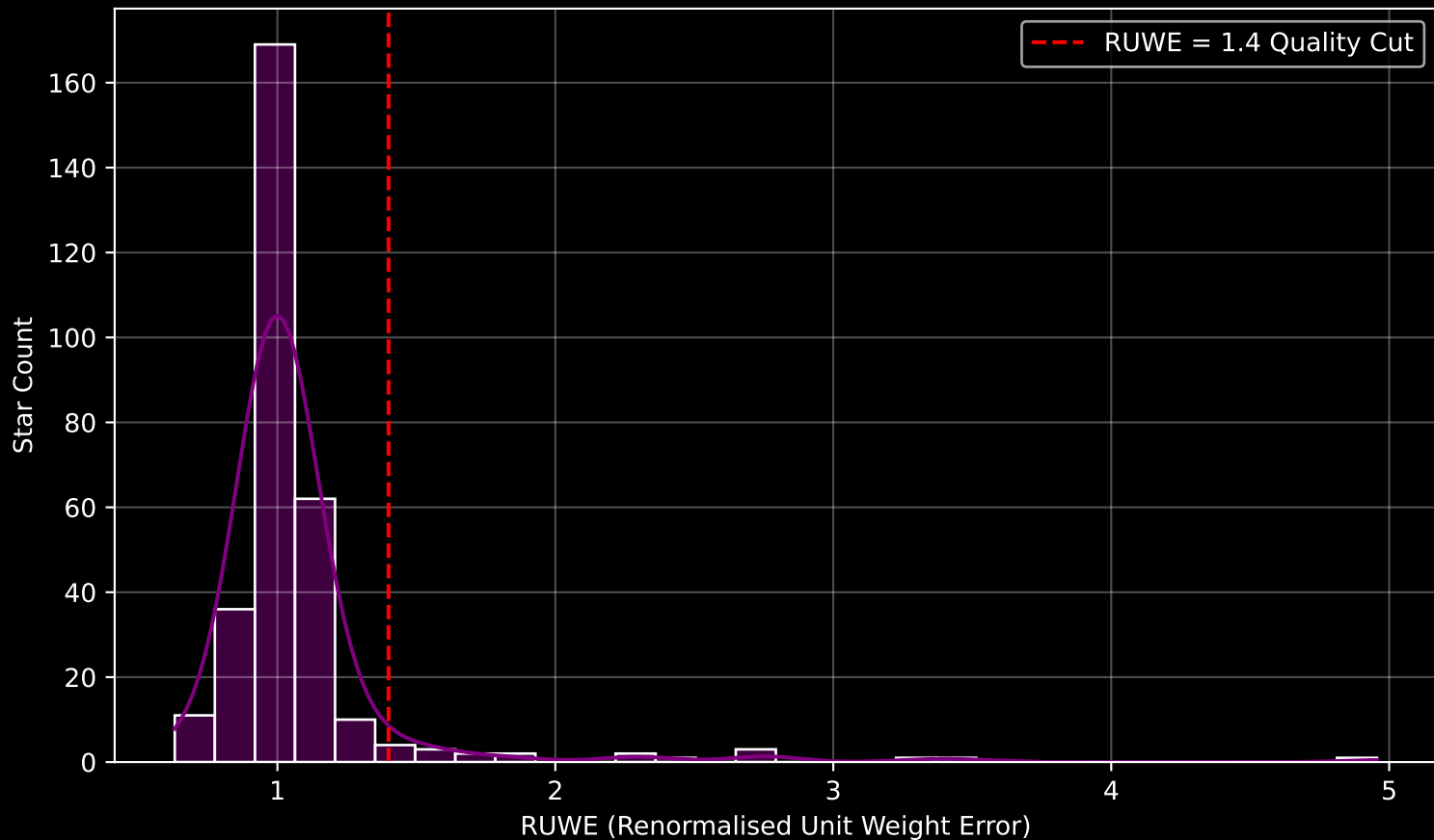
GAPOGEE DR17 Field [000-04-O] RUWE Distribution (n= 308)
