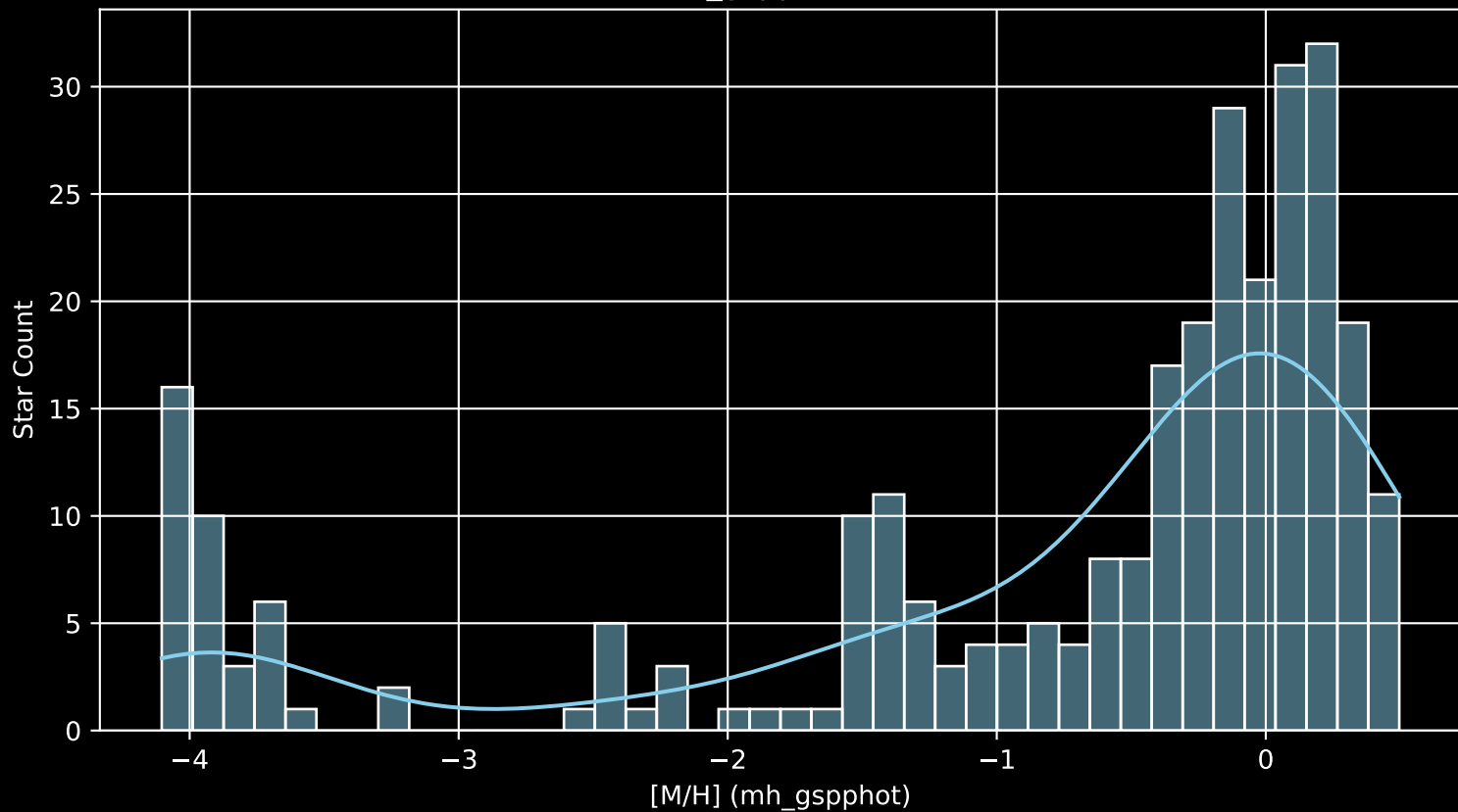
APOGEE DR17 Field: [000-04-O [M/H] (mh_gspphot) (n= 294)
